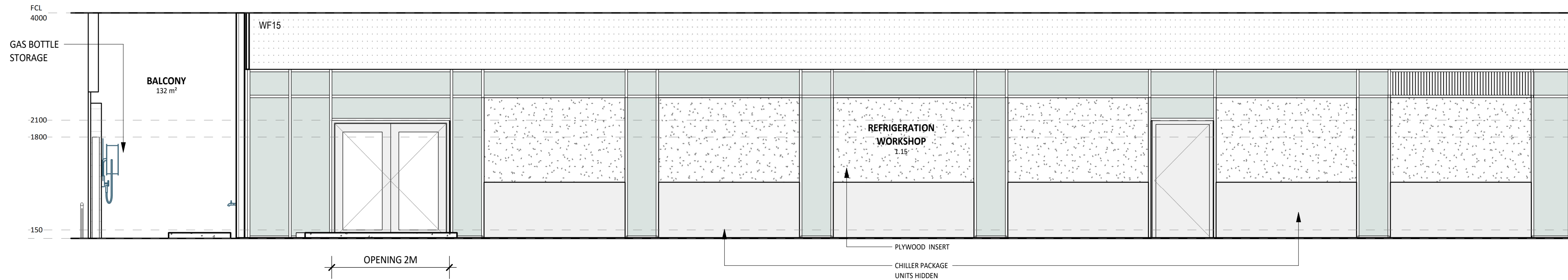
3 ELEVATION DETAIL 60-039 1 : 50
