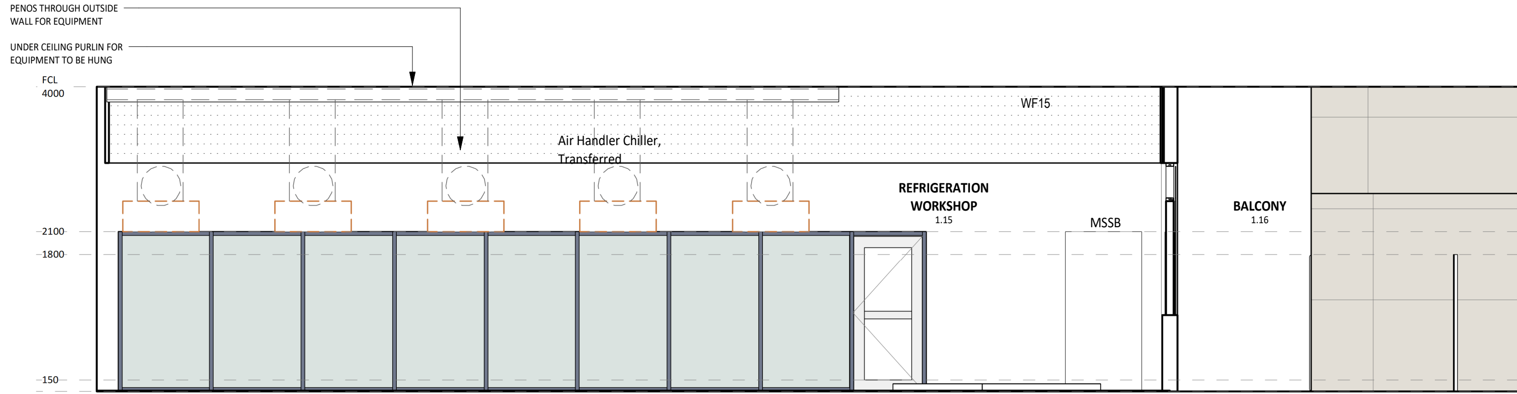
2 ELEVATION DETAIL 60-039 1 : 50
